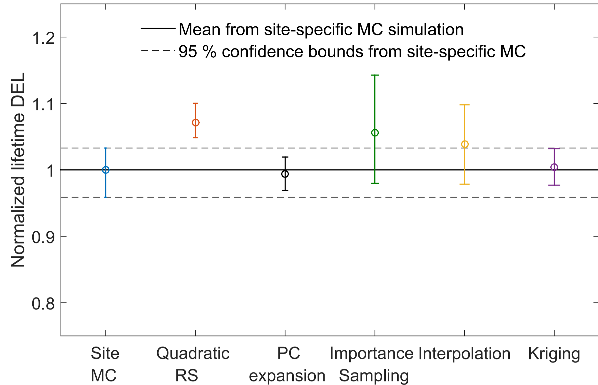
Tower base fore-aft M_x lifetime DEL: mean and 95 % CI estimates, reference site #0
