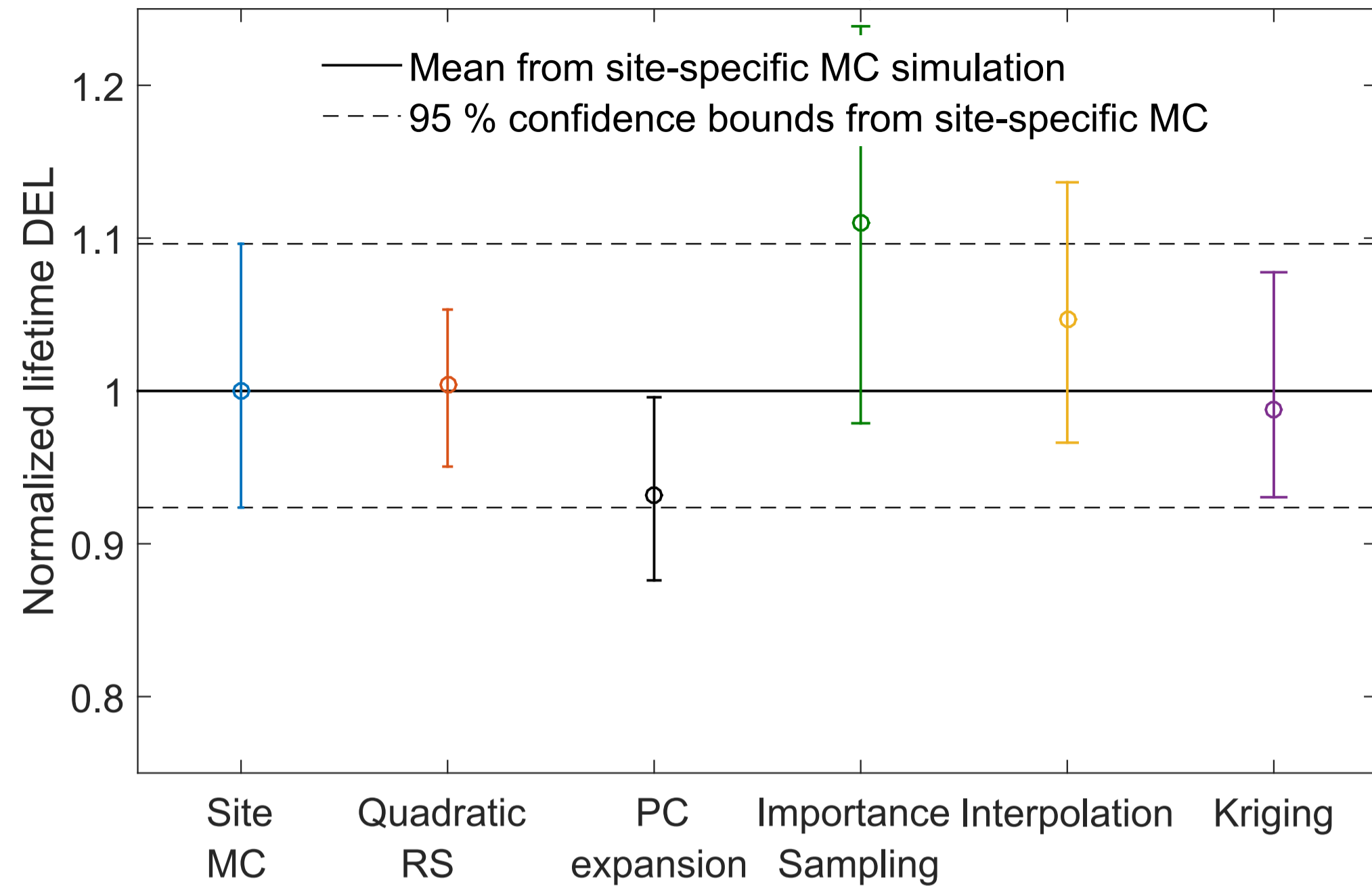
Tower base side-side M_y lifetime DEL: mean and 95 % CI estimates, reference site #0
