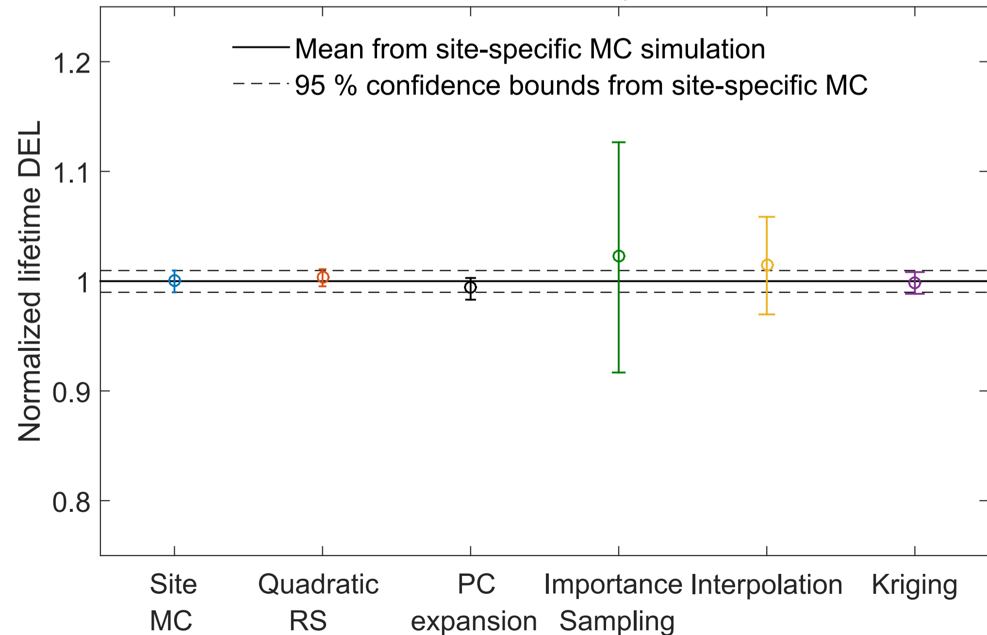
Tower top fore-aft M_x lifetime DEL: mean and 95 % CI estimates, reference site #0
