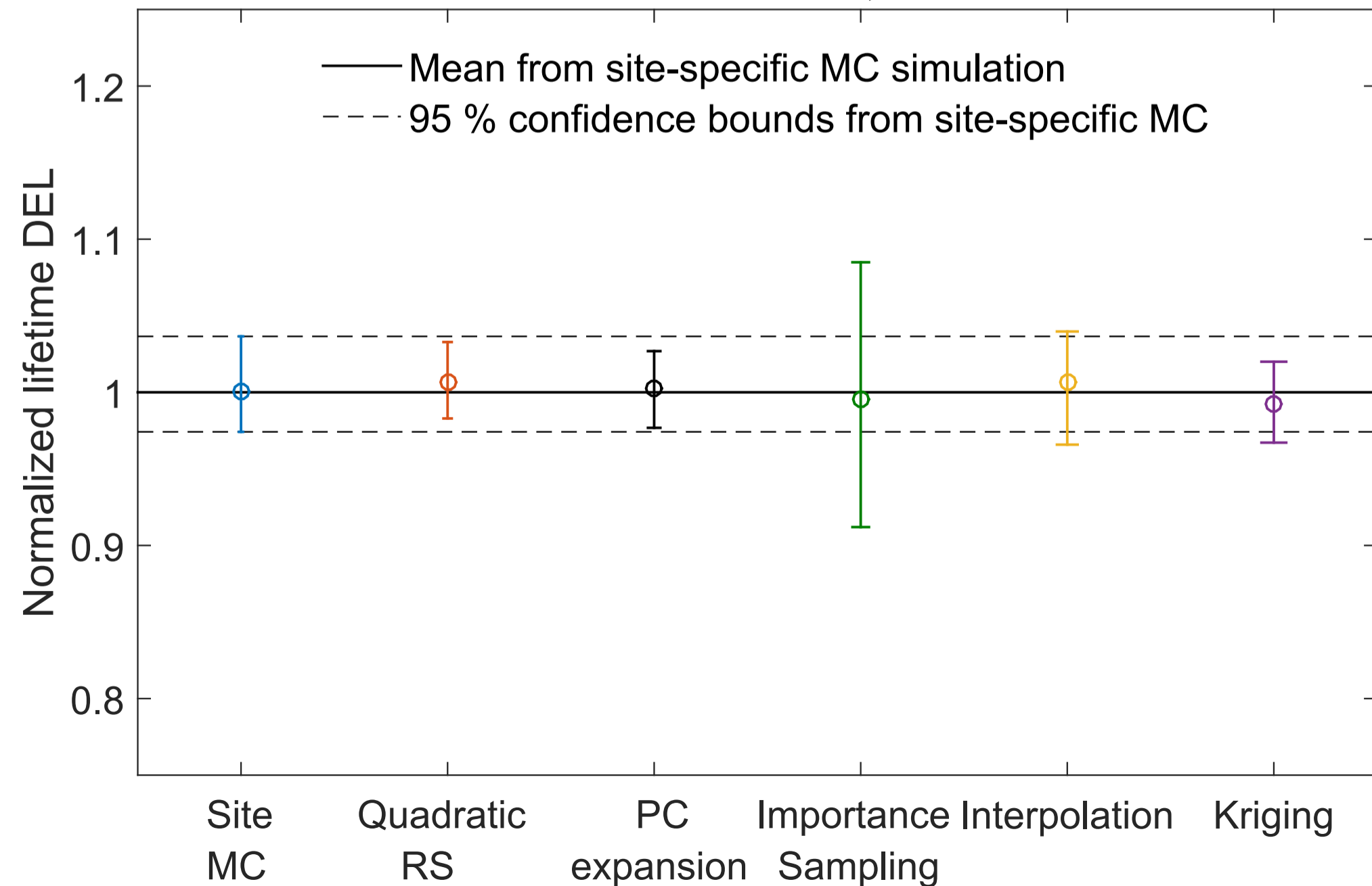
Tower top side-side M_y lifetime DEL: mean and 95 % CI estimates, reference site #0
