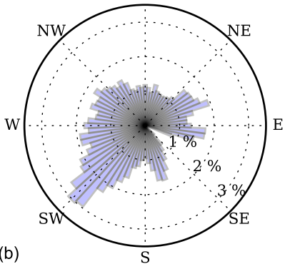
NoordzeeWind wind rose
